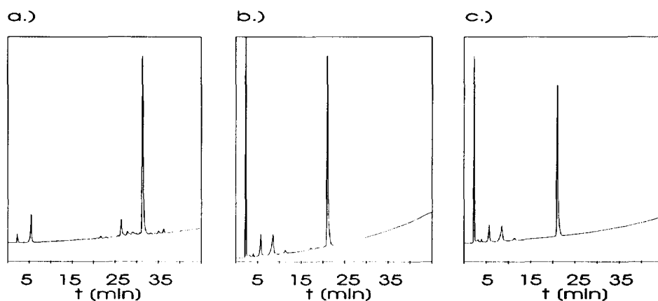
Figure 2. HPLC-profiles of protected alamethicin F30 (ES-MS: calcd. for [M+H]^+ : 2505.0 found: 2505.5) (a), and of crude alamethicin after final deprotection for 30 min (ES-MS: calcd. for [M+H]^+ : 1964.3 found: 1965.7) (b) and 240 min (c).
