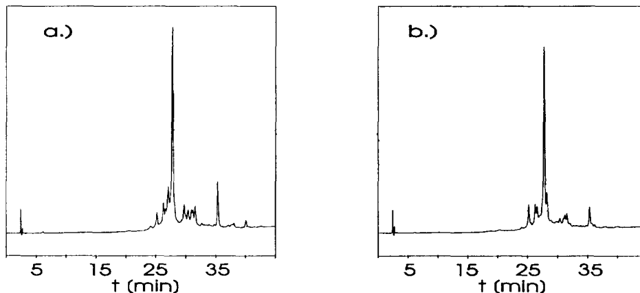
Figure 3. Syntheses of chloroac-Gly-BOVTESTIS (345-365) by conventional synthesis via TBPIPU (ES-MS: calcd. for [M+H]^+ : 2511,3 found: 2510,2)(a) and by MPS via fluorides (ES-MS: calcd. for [M+H]^+ : found: 2509,9) (b).
